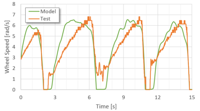
Figure 9: Simulation model validation.
