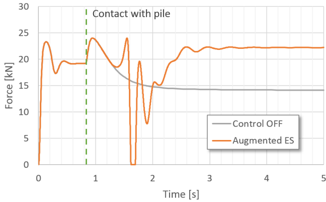
Figure 11: Longitudinal force for vehicle simulation in high-friction condition.
