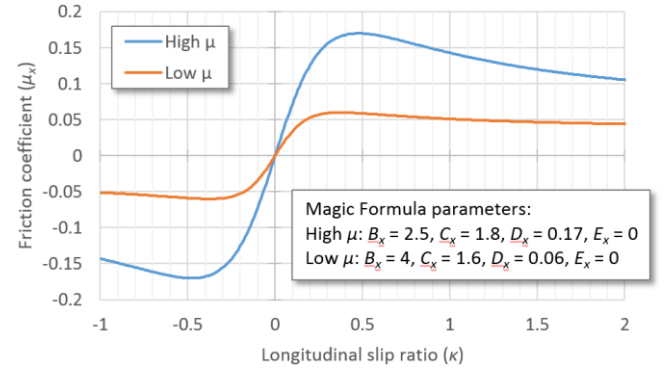
Figure 4: Example Magic Formula plots.
