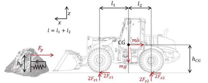
Figure 2: Wheel loader force diagram.
